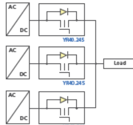
N+1-Redundancy
