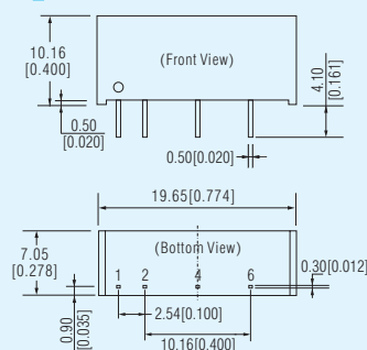
B_S-3WR2 Series (SIP) LxWxH: 19.65x7.05x10.16(mm)
