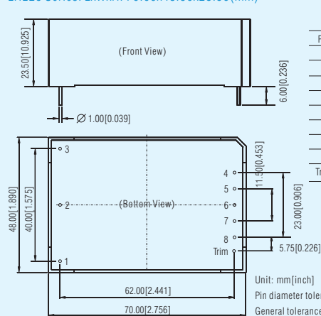
LHE25 Series: LxWxH: 70.00x48.50x23.50(mm)
