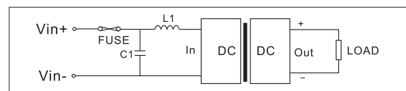
Simple overload protection
