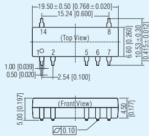
IF_RT-1W Series LxWxH: 19.50x10.53x5.00(mm)
