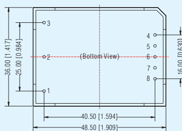
Pin-Out
