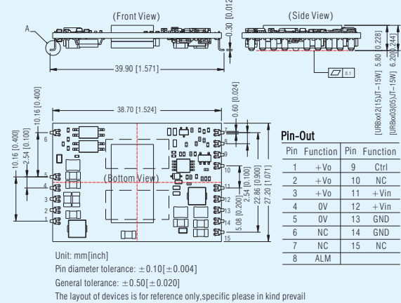
URB_JT-15W (Open frame, SMD package) LxWxH: 38.70x27.20x6.20(mm)
