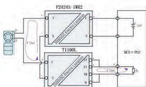
Fig 10. Sample Two - the wiring diagram of the Passive Series Conditioning Module
