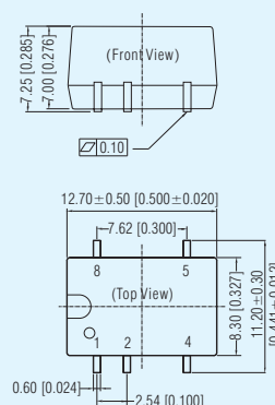
B/F_XT-2WR2 Series LxWxH: 12.70x11.20x7.25(mm)
