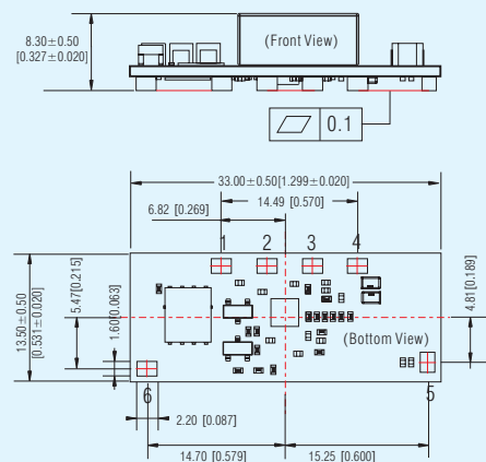
K12T-10A, 16A Series LxWxH: 33.02x13.50x8.32(mm)
