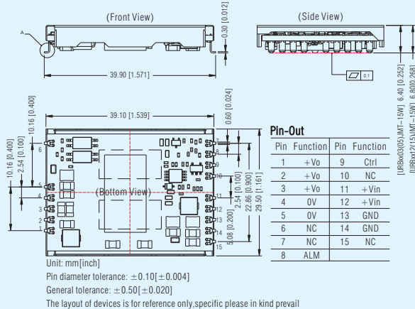
URB_JMT-15W (SMD package with shell) LxWxH: 39.10x29.50x6.80(mm)
