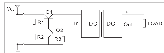
Figure 3: Continuous over current protection circuit
