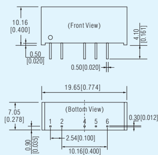
E_S-2WR2, F_S-2WR2, F_S-3WR2 Series(SIP) LxWxH: 19.65x7.05x10.16(mm)
