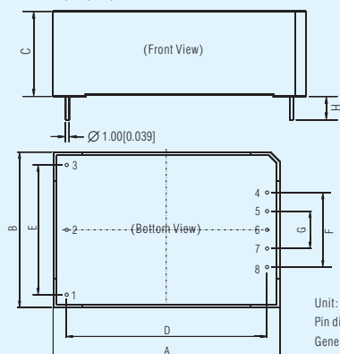
Pin-Out
