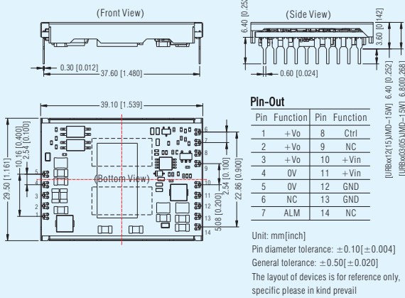
URB_JMT-15W (SMD package with shell) LxWxH: 39.10x29.50x6.80(mm)
