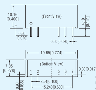
E_S-2WR2, F_S-2WR2, F_S-3WR2 Series(SIP) LxWxH: 19.65x7.05x10.16(mm)
