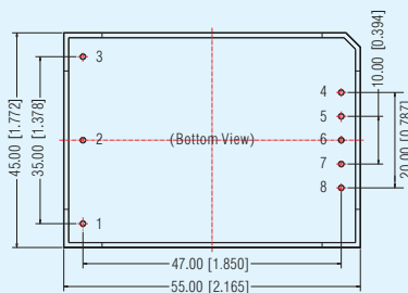
Pin-Out
