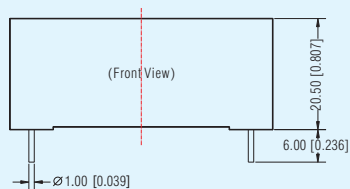
LHE05-20A/C/Dxx Series: LxWxH: 48.50x36.00x20.50(mm)
