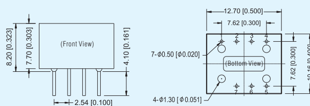
TD5(3)01MCAN(FD) Series LXWXH: 12.70x10.16x7.70(mm)
