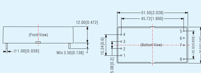
TDH501DCAN-ZC Series; LxWxH: 51.5X26.50X12.00(mm)
