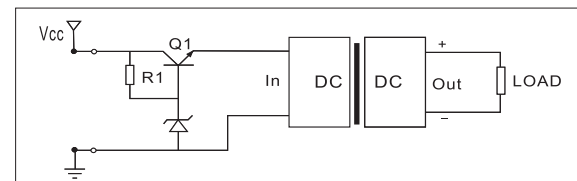
Figure 2: Continuous over voltage protection circuit
